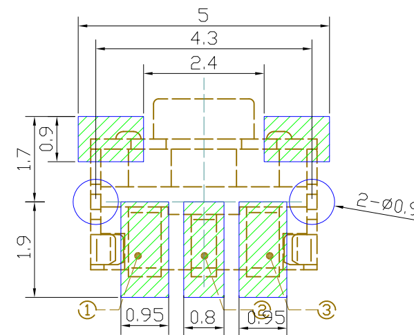
P. C. B MOUNTING PATTERN DIMENSION the following soldering are recommended for reflow soldering
