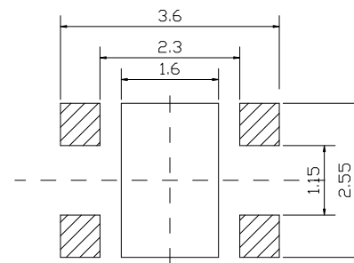
PCB.circuit prohibited area
